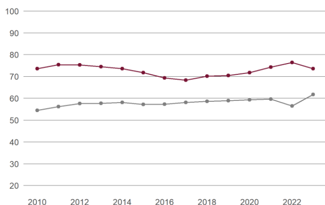
Historie ESG-Score
